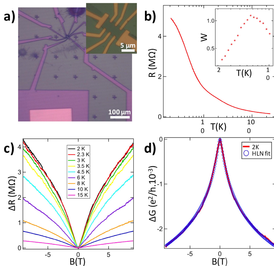
Figure 6. Electrical data of monolayer 1T' - WTe_2 . (a) Optical image showing the device structure with a visible window through the PMMA coating to the contact electrode. Inset: Optical micrograph of the monolayer 1T' - WTe_2 flake device. (b) Resistance versus temperature behavior of the device. Inset: Reduced activation energy as a function of temperature showing metallic behavior. (c) Magnetoresistance for different temperatures, showing the appearance of the weak antilocalization cusp. (d) Magnetoconductance measurement at 2 K (red curve), fitted with Hikami–Larkin–Nagaoka (HLN) theory (blue circle). The results show excellent agreement between the data and the fit.
